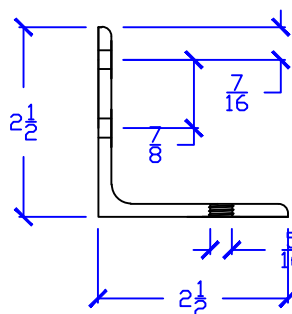
\frac{5}{16} -18 Threaded Hole
